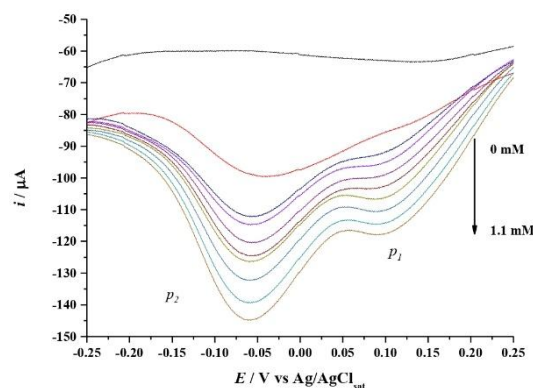
Figure 3: Family of LVs obtained in the system 0.1 M acetate buffer at pH=5, with different Cr (III) concentrations indicated in the figure, using CPE- \beta -CD-EDTA-CS, the potential sweep started at 0.3 V, in the cathodic direction, at 100 \text{ mV s}^{-1} .
