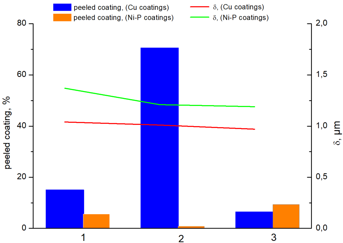
Fig. 1. Comparison of the percentage of coating delamination and the thickness \delta ( \mu\text{m} ) for Cu and Ni–P coatings under different \text{SnO}_2 deposition conditions:
