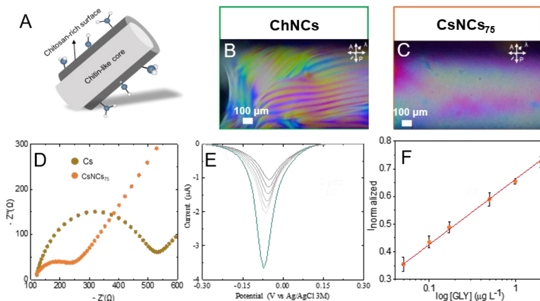
Figure 1. A ) Schematic representation of the chitosan-rich surface and the chitin-like core. POM images of glass capillaries loaded with suspensions of B ) ChNCs, and C ) CsNCs 75 . D ) Zoomed-in Nyquist plot recorded in 1:1 2.5 mM ferro/ferricyanide mixture, 0.15 M Britton-Robinson buffer (pH 6) at the open circuit potential. E ) Calibration response and F ) Calibration plot reporting the normalized peak current versus the logarithm of GLY concentration in solution.
