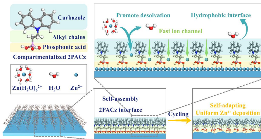
Scheme 1. Schematic diagram illustrating the functional zoning mechanism of the 2PACz interfacial layer.
