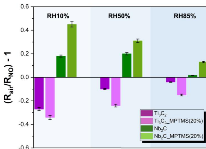
Figure 2. Comparison of sensors signals obtained with pristine and modified MXenes at different RH%, toward 5 ppm of NO (operating temperature = 25 °C; average values on three replicates).
